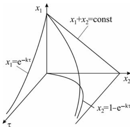
FIGURE 2.5. Kinetics and material balance constraints in chemical system.
