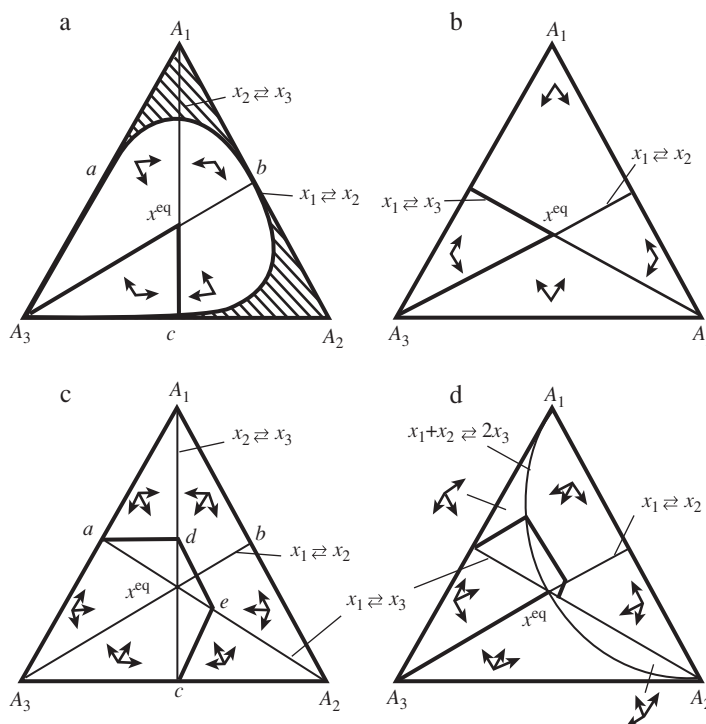
FIGURE 1.2. A graphical interpretation of the algorithm of search for attainable states of a thermodynamic system at a given mechanism of the process.
