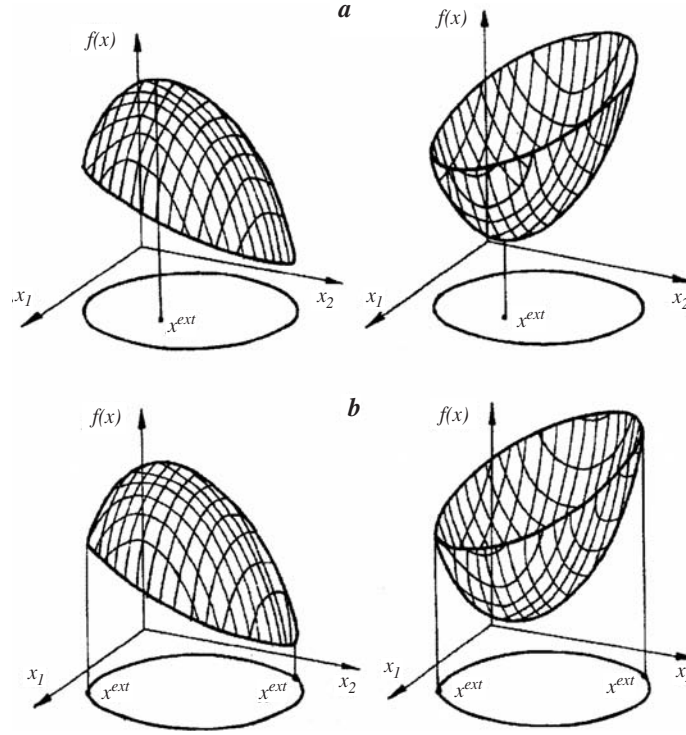
FIGURE 2.1. A graphical interpretation of the problems of convex (a) and concave (b) programming.
