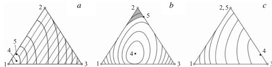
FIGURE 5.22. Steam conversion of carbon. Vertices: 1 – \text{y} : \text{C}, \text{H}_2\text{O} ; 2 – \text{CH}_4 ; 3 – \text{CO}, \text{H}_2 . Thermodynamic states: 4 – x^{\text{eq}} , 5 – x_{\text{CH}_4}^{\text{ext}} . Thermodynamic parameters: P = 5 MPa; T , K: a) 700, b) 800, c) 900. The region of thermodynamic inaccessibility is hatched.
