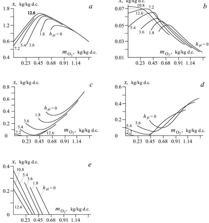
FIGURE 5.25. Plasma gasification of coal. Specific yields of (a) carbon oxide x_{\text{CO}} , (b) hydrogen x_{\text{H}_2} , (c) carbon dioxide x_{\text{CO}_2} , (d) water vapor x_{\text{H}_2\text{O}} , and (e) condensed carbon x_{\text{C}_c} as functions of oxygen consumption m_{\text{O}_2} at different plasma energy values h_{pl} , MJ/kg d.c. ( m_{\text{H}_2\text{O}} = 0.114 \text{ kg/kg dry coal} ).
