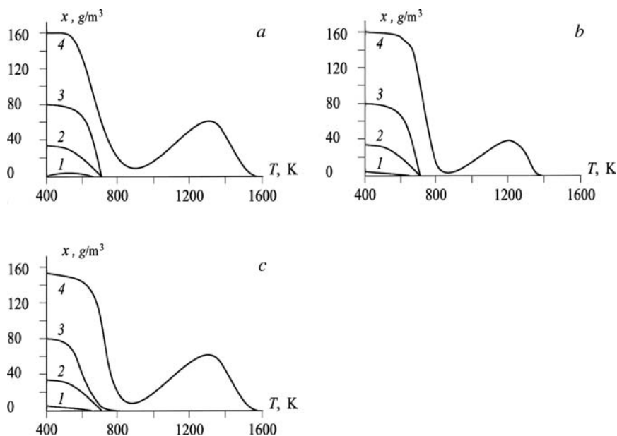
FIGURE 5.20. Equilibrium PAH concentrations versus combustion temperature at different air excesses. a ) \text{C}_{14}\text{H}_{10} , anthracene gas; b ) \text{C}_{14}\text{H}_{10}:\text{c} , condensed anthracene; c ) \text{C}_{14}\text{H}_{10} , phenanthrene gas. \alpha_{\text{air}} : 1, 0.4; 2, 0.3; 3, 0.2; 4, 0.1.
