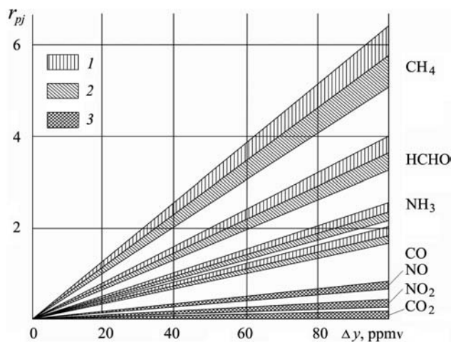
FIGURE 5.3. Relative responses of the atmosphere to emission of particular pollutants (the pollutants are denoted on the right). Secondary pollutants: 1—organic, 2—inorganic, 3—organic and inorganic.
