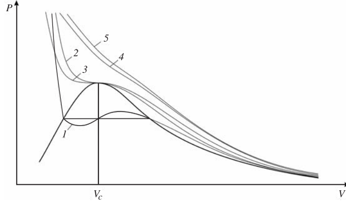
FIGURE 2.10. Isotherms and regions of convexity: P, V - diagram of ideal and real gases. 1, 2, 4: the van der Waals gas ( 1 - T < T_c ; 2 - T = T_c ; 4 - T = 1.148T_c ); 3, 5: the Redlich-Kwong gas ( 3 - T = T_c ; 5 - T = 1.111T_c ).
